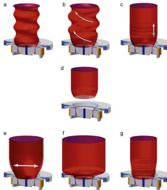
Fig. 2. Different types of bubble instabilities in film blowing process: (a) draw resonance, (b) helical instability, (c) FLH instability, (d) bubble tear, (e) bubble breathing, (f) bubble sag and (g) bubble flutter.
